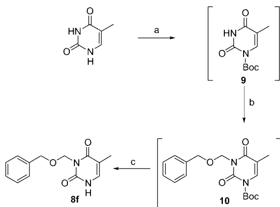
Scheme 2. Synthesis of N 3-(benzyloxymethyl)thymine. (a) Di- tert -butyl dicarbonate, DMAP, CH 3 CN, room temp., 4 h; (b) NaH, BOM-Cl, DMF, room temp., 1 h; (c) K 2 CO 3 , MeOH, room temp., 2 h.
