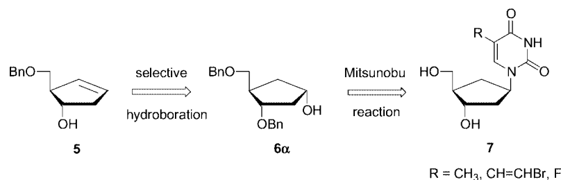
Figure 2. Convergent synthesis of carbocyclic nucleosides starting from a chiral cyclopentanol.
