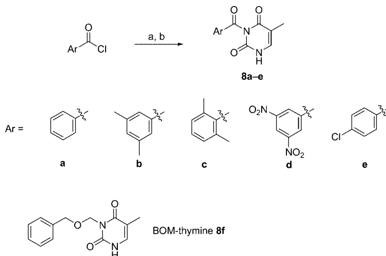
Scheme 1. Synthesis of different N 3-benzoylthymine derivatives 8 . (a) Thymine, pyridine, CH 3 CN, room temp., 2 d; (b) chromatography on silica gel (CH 2 Cl 2 /MeOH, 20:1).
