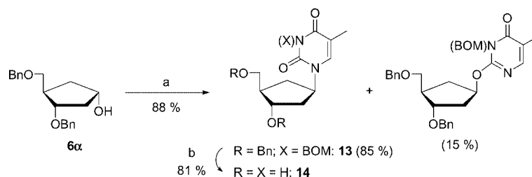
Scheme 4. Application of the N 3-BOM method to the synthesis of carba -dT. (a) \text{PPh}_3 , DIAD, N 3-(benzyloxymethyl)thymine ( 8f ), \text{CH}_3\text{CN} , -40^\circ\text{C} to room temp., 16 h.
