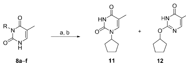
Scheme 3. Coupling of the N 3-protected thymine with cyclopentanol. (a) PPh 3 , DIAD, cyclopentanol, THF, –40 °C to room temp., 16 h; (b) 1% NaOH in MeOH, room temp., 12 h.
